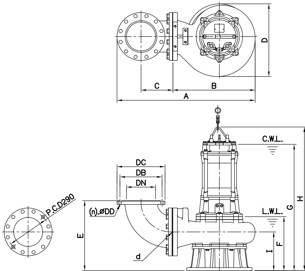
Dimensions—mm
